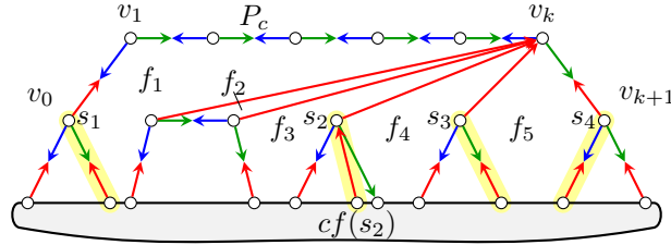
Figure 4: Illustration for some of the definitions used in the proof of Theorem 1. The situation if P_c is a path. The edges that we add to D are marked in yellow. In the depicted situation, v_1 v_2 is not in H .
